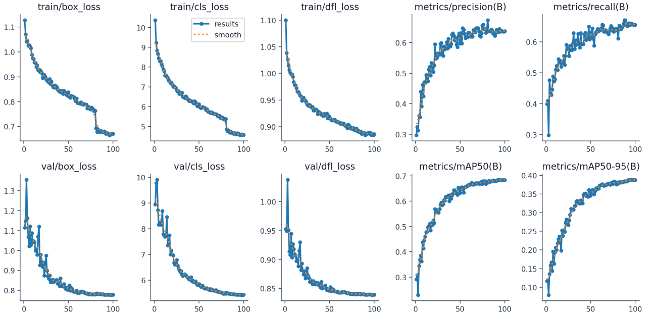
Figure 4: Training dynamics over 100 epochs
