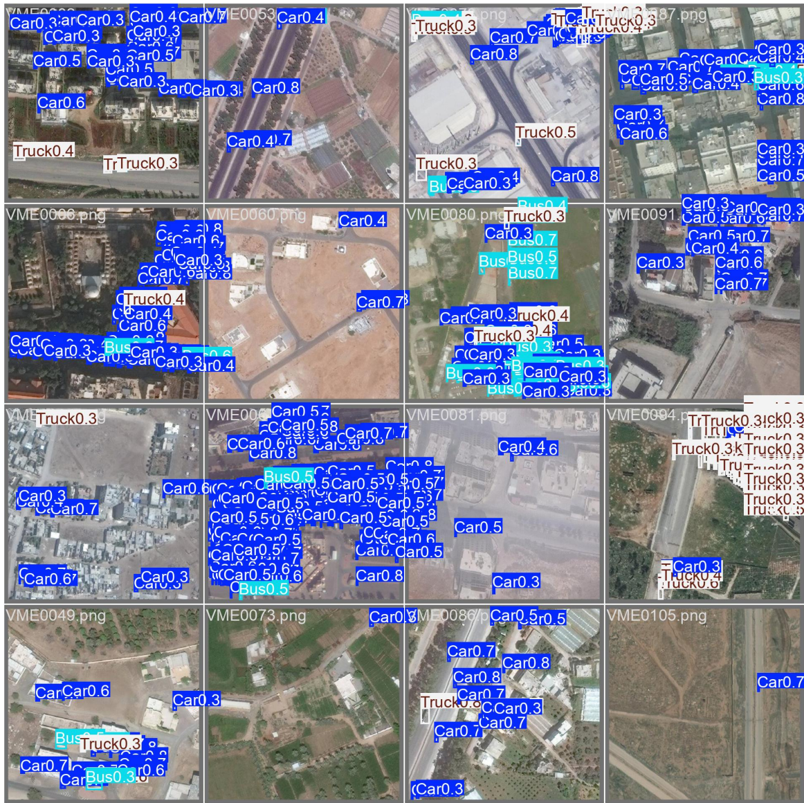
Figure 6: Model predictions on the corresponding validation batch
