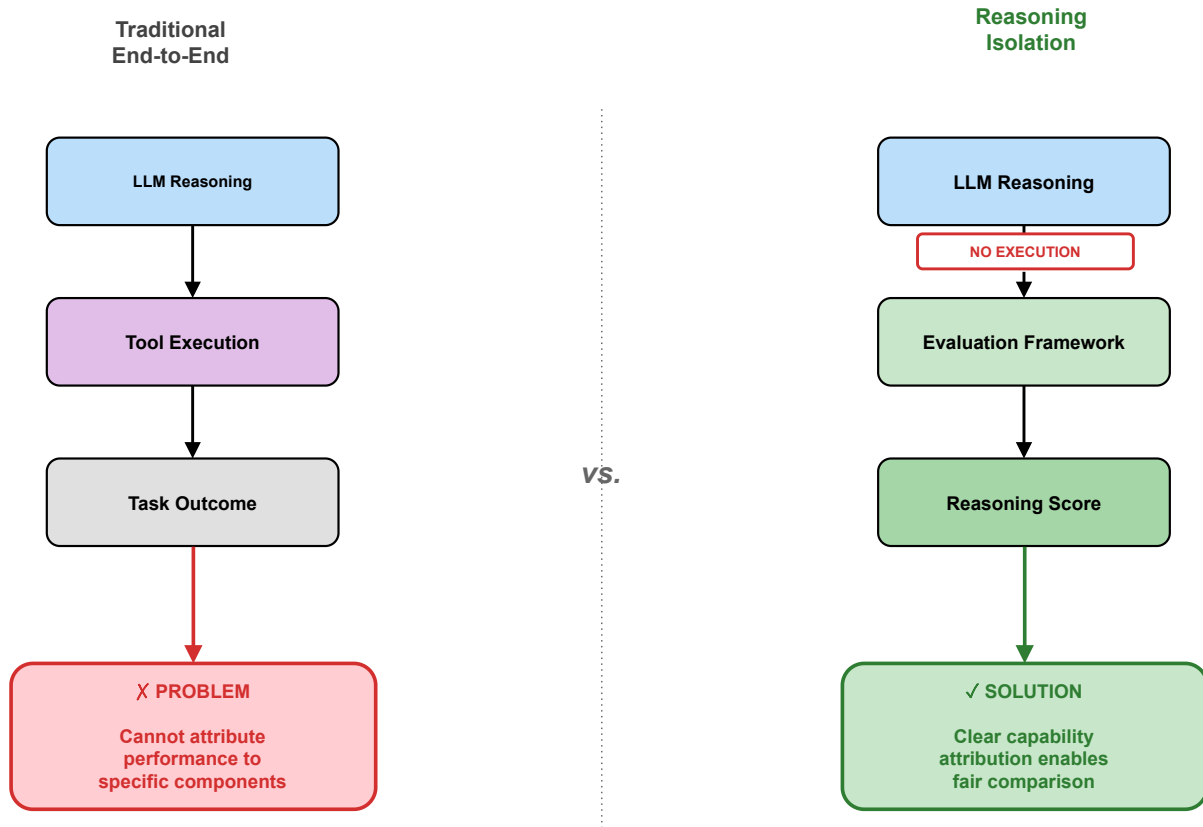
Figure 1: Conceptual comparison between traditional end-to-end evaluation and the proposed execution-free framework. The proposed approach isolates LLM reasoning from execution and environmental factors.
